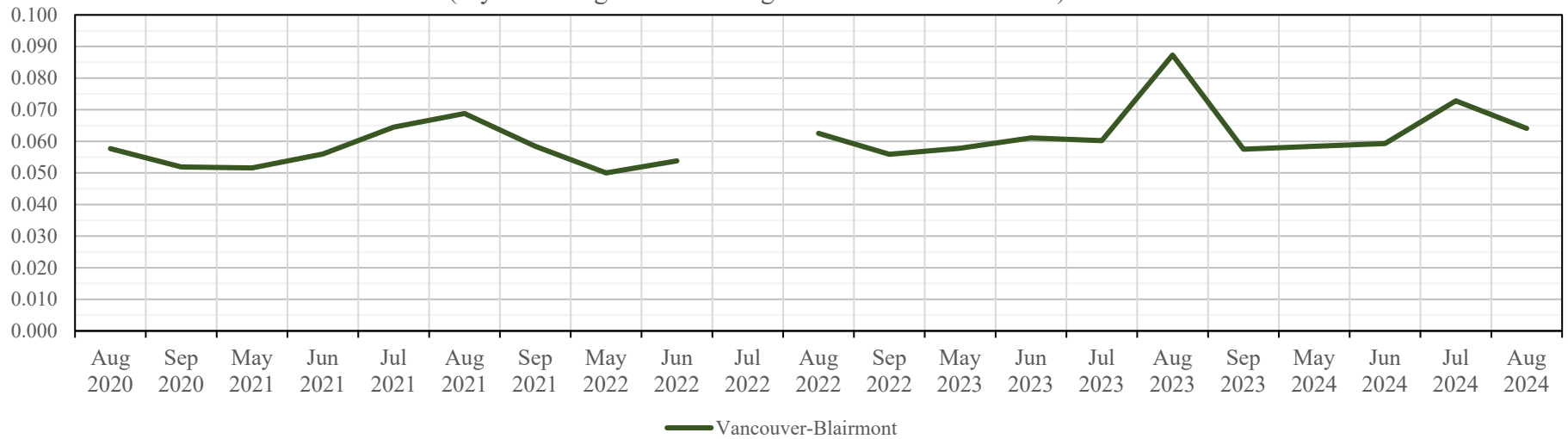
Ozone - Max 8-hour Averages - ppm National Standard - 0.070 ppm (3-year average of the 4th highest 8-hour annual values)
