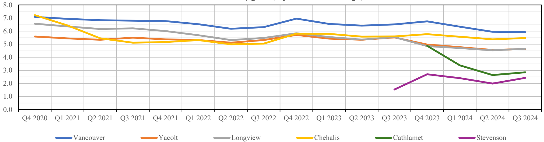
PM 2.5 - rolling annual averages - \mu\text{g}/\text{m}^3 [excludes flagged wildfire days] National Standard - 9 \mu\text{g}/\text{m}^3 (3-year annual average)
